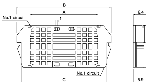
(21, 23, 25, 27, 29, 31 circuits)
