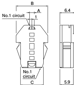
(3 circuits)
