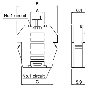
(5, 7 circuits)
